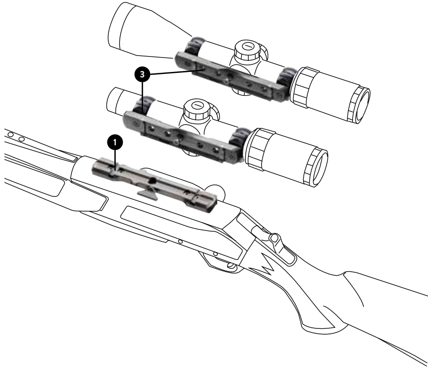
BROWNING NOMAD SINGLE MOUNT
